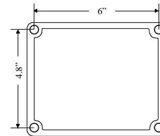
MOUNTING DIMENSIONS
